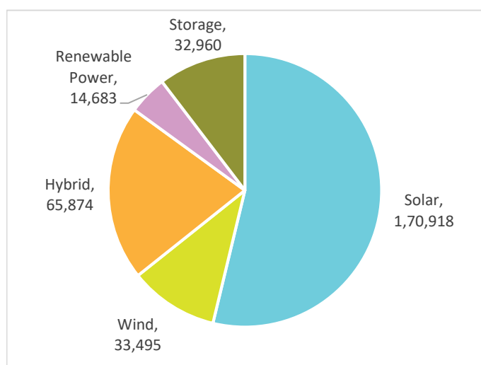
Exhibit 9: Total ~317GW in tendering stage (figures in MW)
