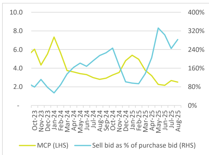
Exhibit 17: Solar hours' supply >280%; MCP stays low
