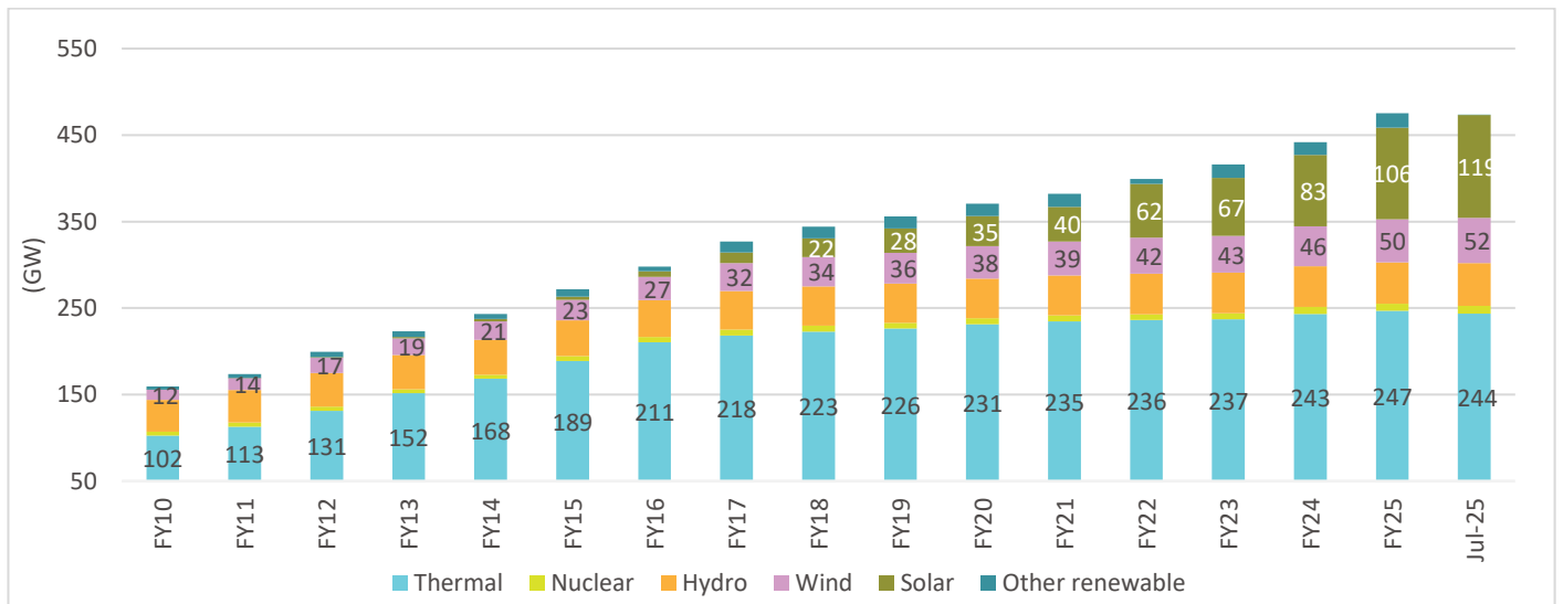
Exhibit 26: Installed capacity till end-Jul-25 at ~490GW – Solar leads the rise FY26 to date
