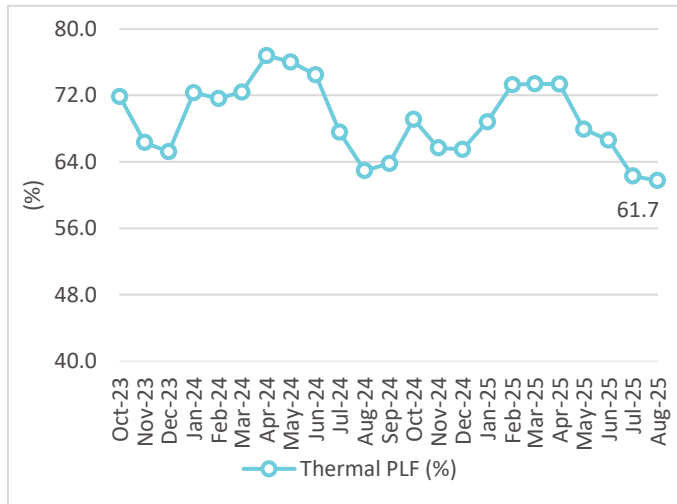
Exhibit 24: Thermal PLF: Aug-25 at 61.7% versus 62.9% YoY
