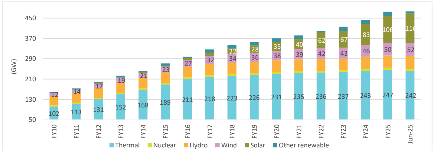
Exhibit 26: Installed capacity in Jun-25 at ~485GW
