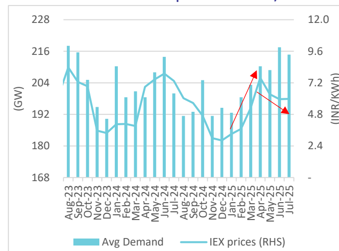
Exhibit 4: Non-solar hours' IEX prices flat at INR6/kWh
