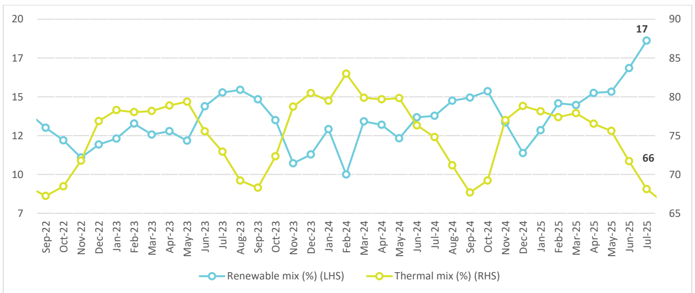
Exhibit 8: Generation: Thermal mix goes down (~66% in Jul-25 versus ~68% in Jun-25); renewable mix at ~17% in Jul-25
