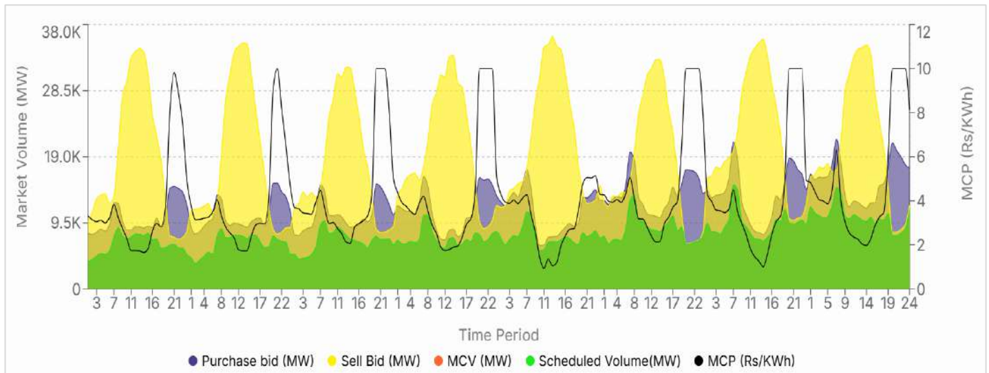
Exhibit 12: IEX prices in Jul-25 hit INR10/kWh cap on 22/31 days while also dipping to as low as INR0.7/kWh
